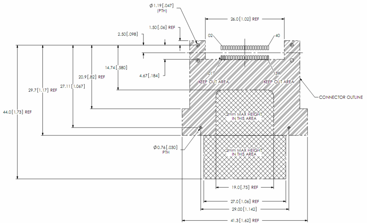
PCB layout for right angle MiniBlade socket
